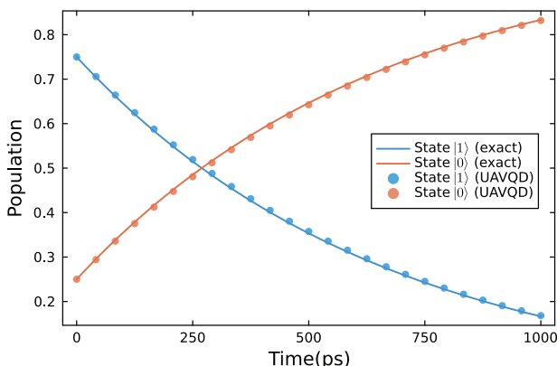
Figure 3. Population comparison between state |0\rangle and state |1\rangle for the amplitude damping model. Solid lines show exact solutions serving as benchmarks, while filled circles represent results from vectorization and UAVQD methods.
