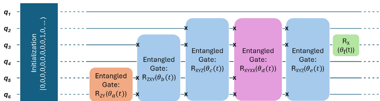
Figure 4. This schematic diagram depicts the part of the quantum circuit utilized in the simulation of the FMO complex, operating with a six-qubit system and with notation same as the previous Figure 2. It highlights the possible arrangements of single-qubit and multi-qubit entangling operations, where cross marks in the blocks represent the qubits involved in an entanglement.
