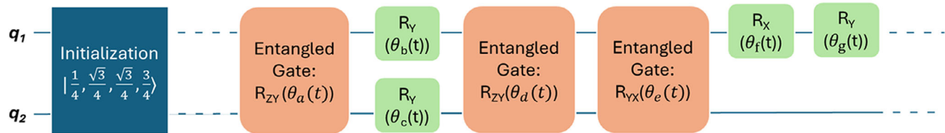
Figure 2. Snippet of the ansatz construction scheme. This figure provides a visual representation of the ansatz used in UAVQD method. The circuit initializes in the state given in first block. Next, the two-qubit entangling operations are labeled as 'Entangled Gate' with notation scheme R_{ZY}\theta_a(t) implies two qubit rotation ZY gate with \theta_a parameter at time t , where subscripts a, b, c, \dots are simply to notify that each block has distinct \theta .
