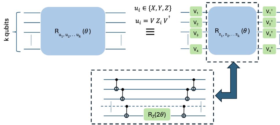
Figure 1. Quantum circuits require the transformation of multi-qubit entangled gates present in the ansatz into CNOT and single-qubit gates. For the general form of the operator present in our ansatz, R_{u_1, u_2, u_3, \dots, u_k} , we first decompose it using the relation u_i = V_i Z_i V_i^\dagger . Here, u_i is one of the Pauli operators, i.e., X, Y, and Z, and their corresponding V are the eigenvectors that diagonalizes the single-qubit unitary into Z . (For example for u_i = X the choice of V_i = H , the conventional Hadamard gate). In the second step, the R_{z_1, z_2, z_3, \dots, z_k} operator in the middle is decomposed into a series of CNOT gates and one R_z gate. With this strategy, we observe a linear scaling of the number of decomposed gates; that is, for every k -qubit entangled gate, we can decompose it into O(k) basis gates.
