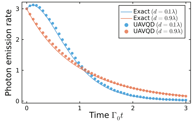
Figure 6. Photon emission rate for the three atom chain configuration is plotted against the time. The solid curves and separated dots represent the exact and UAVQD-vectorization calculations respectively for two possible scenarios: when atoms are densely packed i.e., d = 0.1\lambda and when atoms are separated at an inter-atomic distance of d = 0.9\lambda which is similar to the magnitude of the excitation wavelength of the coupling field. The method was employed with a timestep of 10^{-3} time unit, utilizing operator pool P2 and an adaptive threshold of 10^{-1} .
