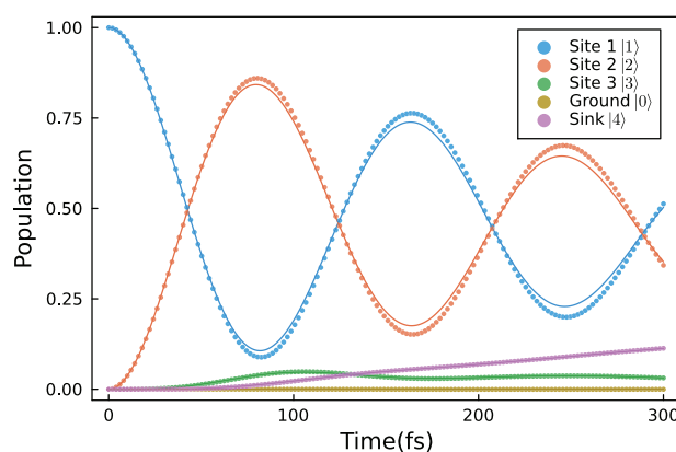
Figure 5. The population dynamics of the FMO complex, showcasing the populations of site 1 through 3, the ground state, and the sink state. The solid lines represent the exact calculations, while the spaced filled dots correspond to calculations using the vectorization and UAVQD methods. The UAVQD method was employed with a timestep of 1 fs, and an adaptive threshold of 10^{-3} .
