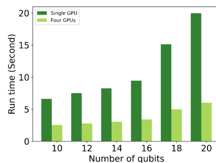
Figure 18. Execution time for an “observe” call (expectation value) made for 10,000 data-points for a one layer of the parametrized quantum circuit similar to the one shown in Figure 16. All simulations were run on an NVIDIA DGX A100 GPU device. For a single GPU, the total 10,000 data-points are dealt within a single GPU (i.e., 10,000 “observe” calls in sequence on a single GPU). For the four GPU case, the data points are split into four batches, each containing 2500 data-points (i.e., 2500 “observe” calls on each GPU).
